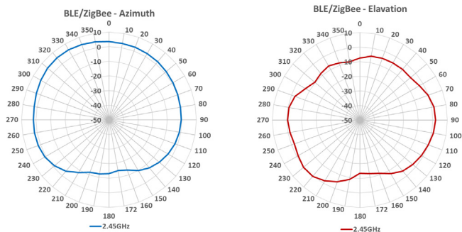
BLE/ZigBee Plot
