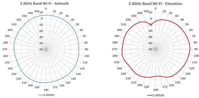
Wi-Fi 2.4GHz Plot
